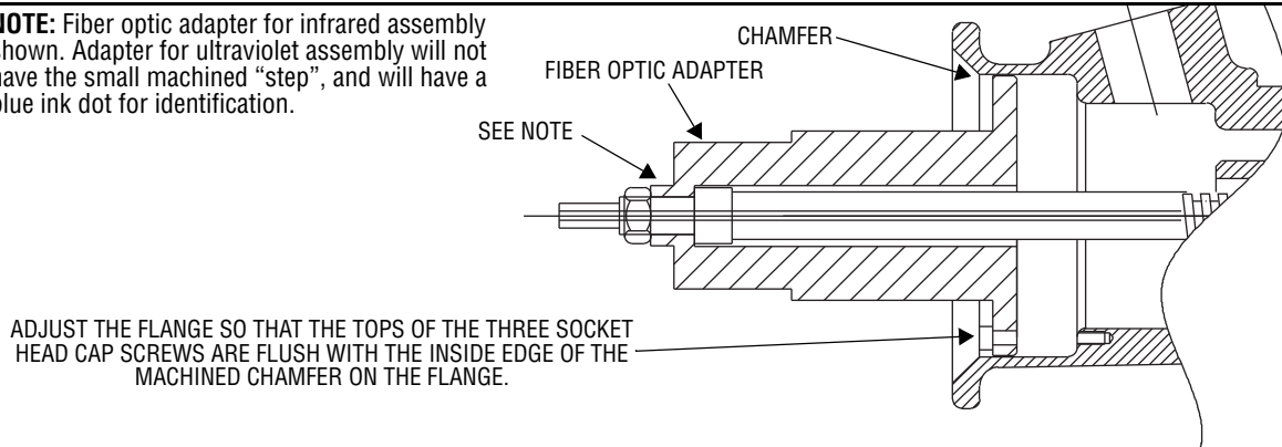
FIGURE 6. ADJUSTING FIBER OPTIC BUNDLE COMPRESSION
