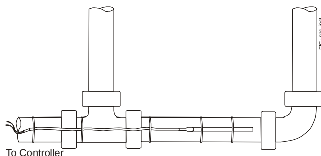
Figure 2: Installing the Strap-Mount Sensor
