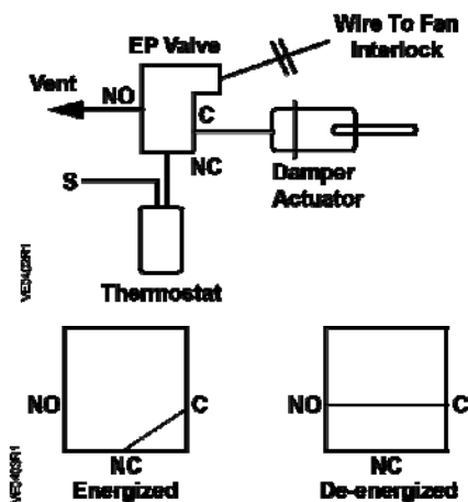
Figure 1. Standard Application.
