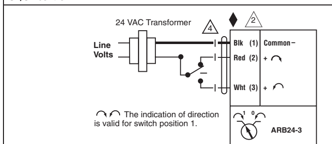
Floating Point or On/Off control
