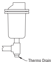
Fig. 2-2. 200 Series trap with Thermo Drain in tee ahead of trap. Trap inlet tube must be removed.
