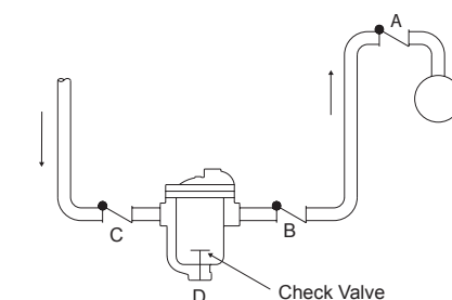
Fig. 1-8. Possible check valve locations.
