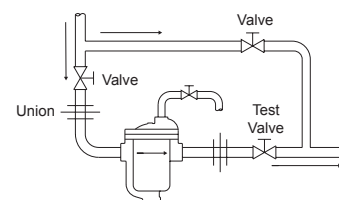
Fig. 1-5. Bypass hookups for No. 800-816 and 880-883 traps.
