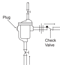
Fig. 1-4. Alternate hookup for No. 800-816 with inlet at bottom and side connection plugged.
