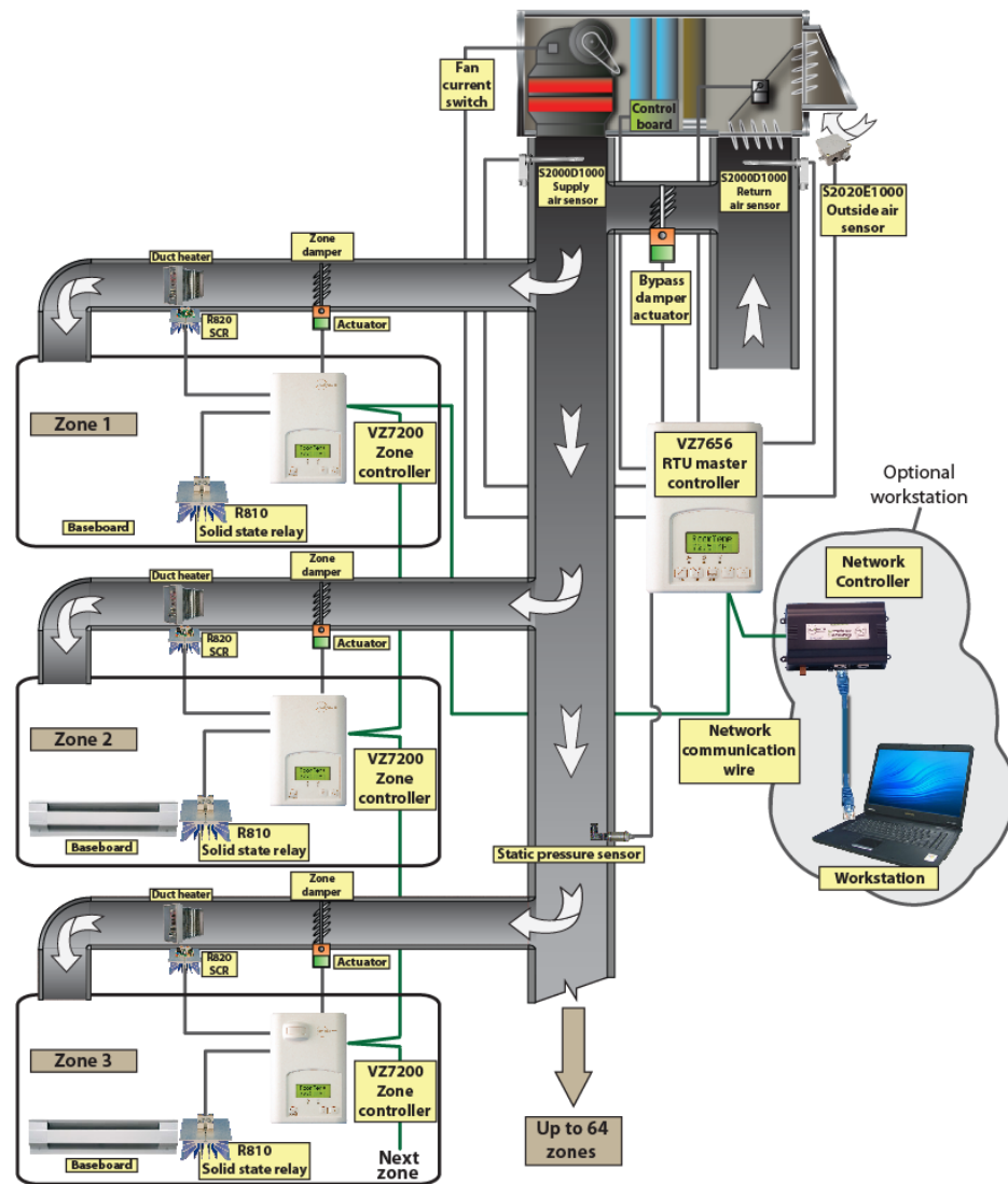
Typical BACnet zoning system installation
