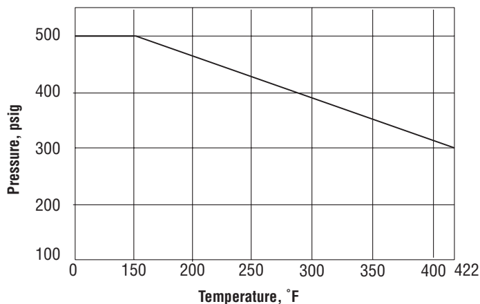
Pressure/Temperature Rating
