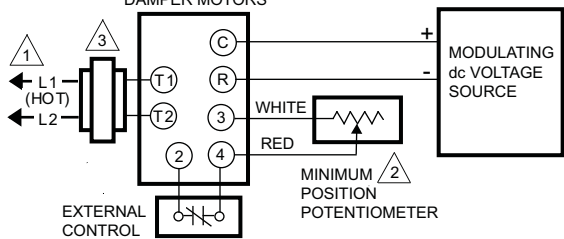
Typical wiring for M7685 motors DAMPER MOTORS
