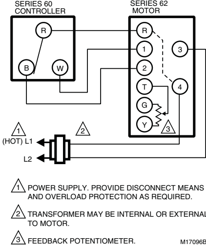
Typical wiring for Series 62 motors
