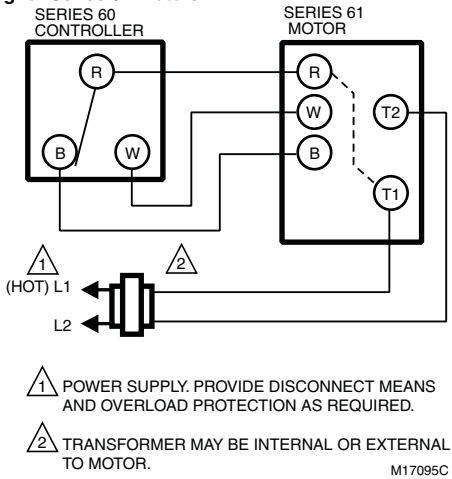
Typical wiring for Series 61 motors
