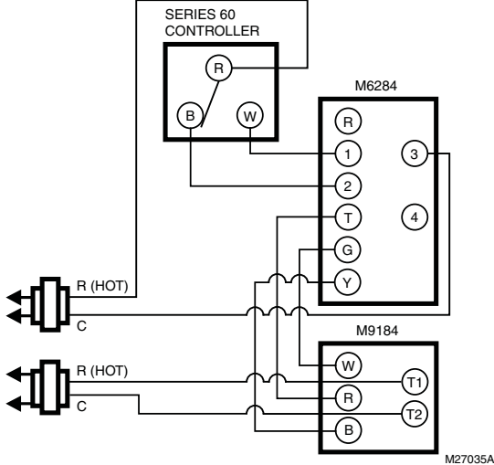
Series 60 and Series 90 motors in slaving application
