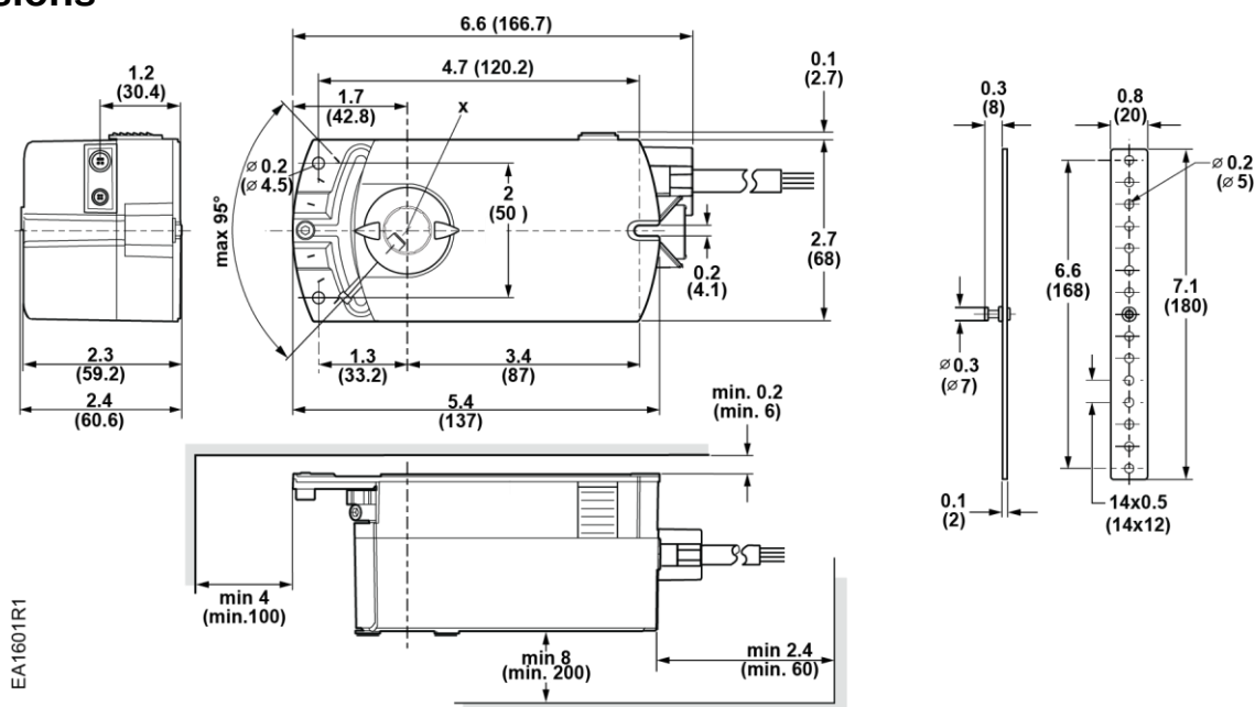
Figure 24. Dimensions of the OpenAir GDE/GLB Enhanced Actuator and Mounting Bracket.
