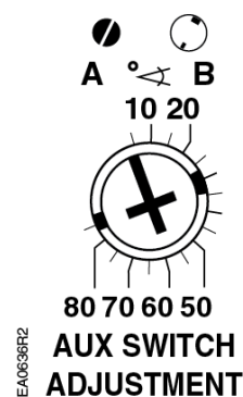
Figure 10. Auxiliary Switch Setting Dial.
