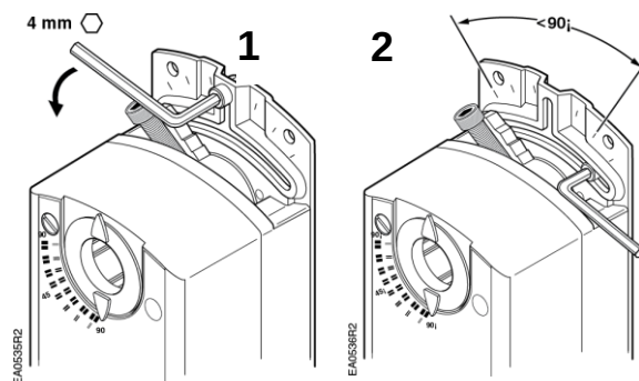
Figure 11. Moving the Mechanical Range Stop.
