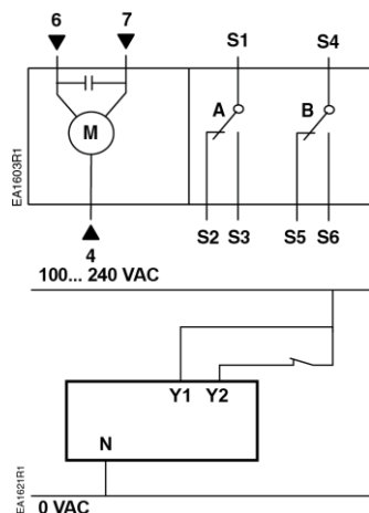
Figure 20. 2-Position, SPST (Single-Pole, Single-Throw).
