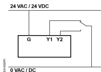
Figure 18. 2-Position, SPDT (Single-Pole, Double-Throw).
