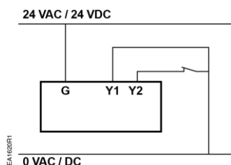
Figure 17. 2-Position, SPST (Single-Pole, Single-Throw).
